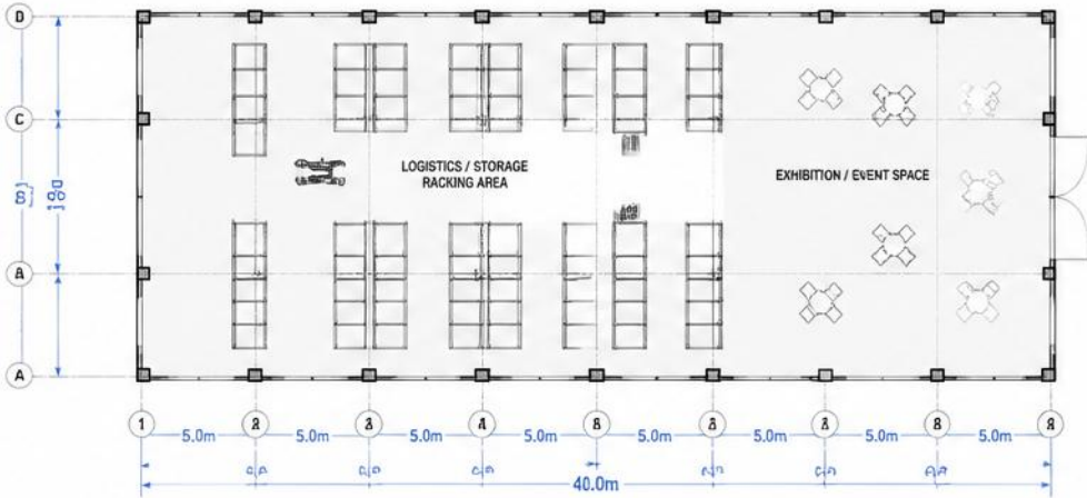
FLOOR PLAN LAYOUT (40.0m x VARIABLE DEPTH)
