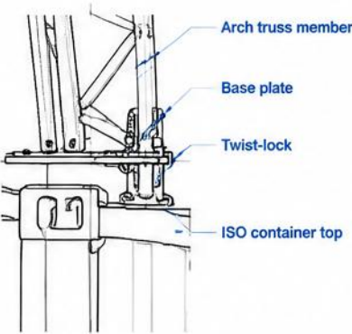
Twist-lock Base Plate Connection Detail (Scale 1:10)
