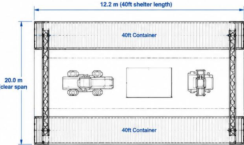
Floor Plan Layout (Scale 1:100)
