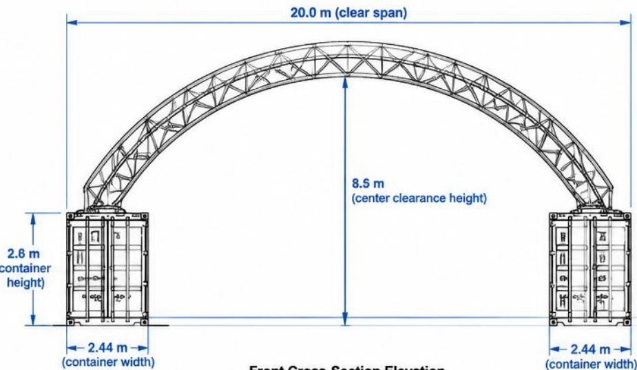
Front Cross-Section Elevation (Scale 1:100)
