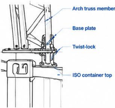
Twist-lock Base Plate Connection Detail (Scale 1:10)
