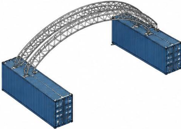
3D Axonometric View (Scale NTS)
