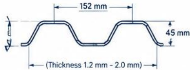
ARCH PROFILE (A-A) (Deep Corrugation, AZ150 Galvalume)
