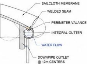
3 PERIMETER DRAINAGE VALANCE DETAIL SCALE 1:10
