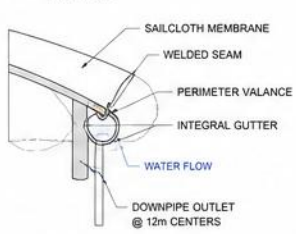
3 PERIMETER DRAINAGE VALANCE DETAIL SCALE 1:10
