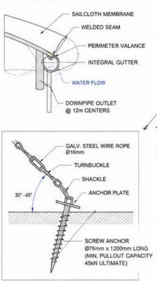
4 EARTH ANCHOR DETAIL SCALE 1:10
