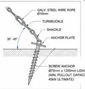
4 EARTH ANCHOR DETAIL SCALE 1:10
