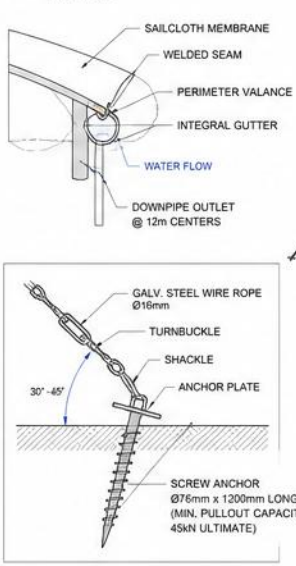
4 EARTH ANCHOR DETAIL SCALE 1:10
