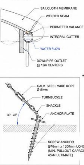
4 EARTH ANCHOR DETAIL SCALE 1:10
