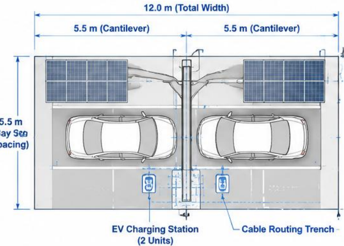
Site Layout Plan (Top View) Scale: 1:100
